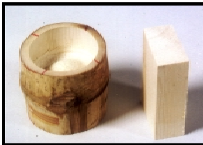
Fig. 42: Bamboo and timber pieces with the same area of cross-section
