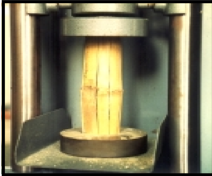
Fig. 48: Bamboo in compression between steel plates
