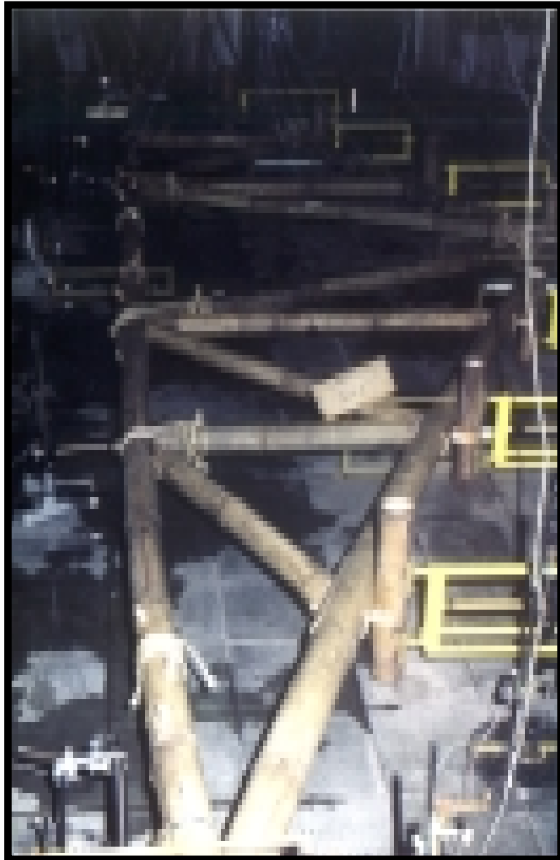
Fig. 53: A truss under test
