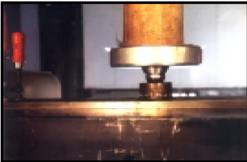
Fig. 49: A reliable compression test using friction-free plates
